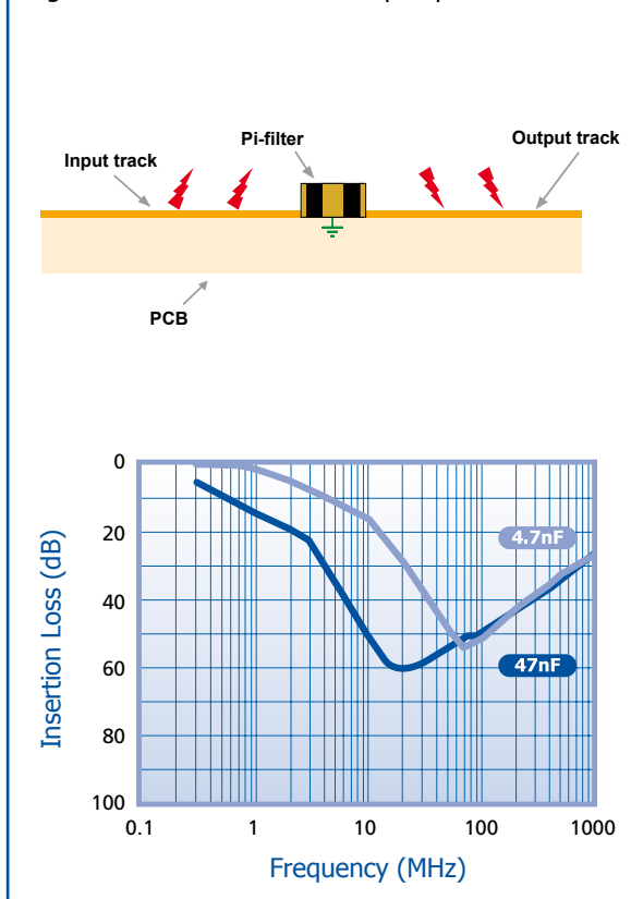
Figure 1. Filters mounted on open pcb
