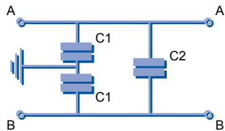
Circuit configuration
