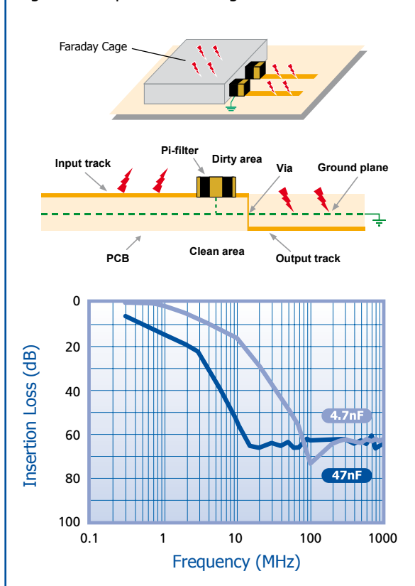
Figure 2. Improved shielding
