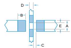
Recommended solder lands
