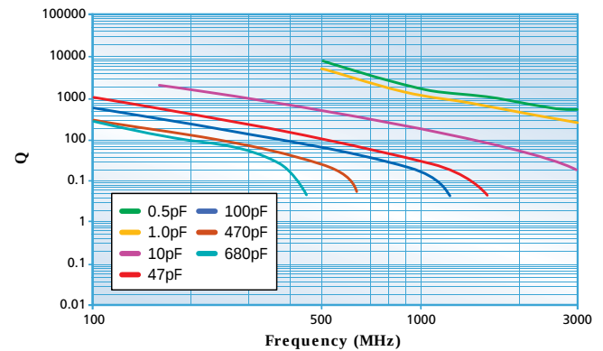
Q(MS) Series Q vs. Frequency - Case size 1111
